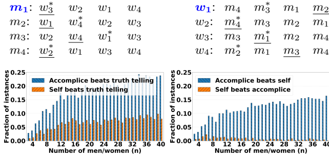
Figure 1: Comparing no-regret accomplice and self manipulation against truthful reporting (left) and against each other (right).
